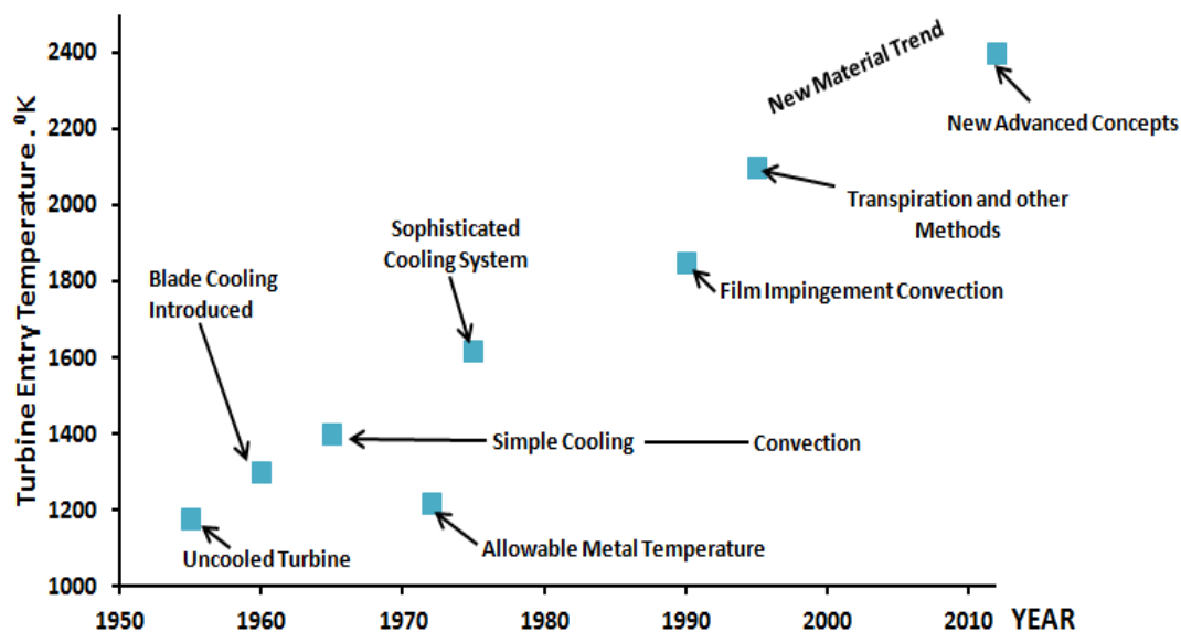
Figure 2.7: Development of cooling technology in gas turbine blade
