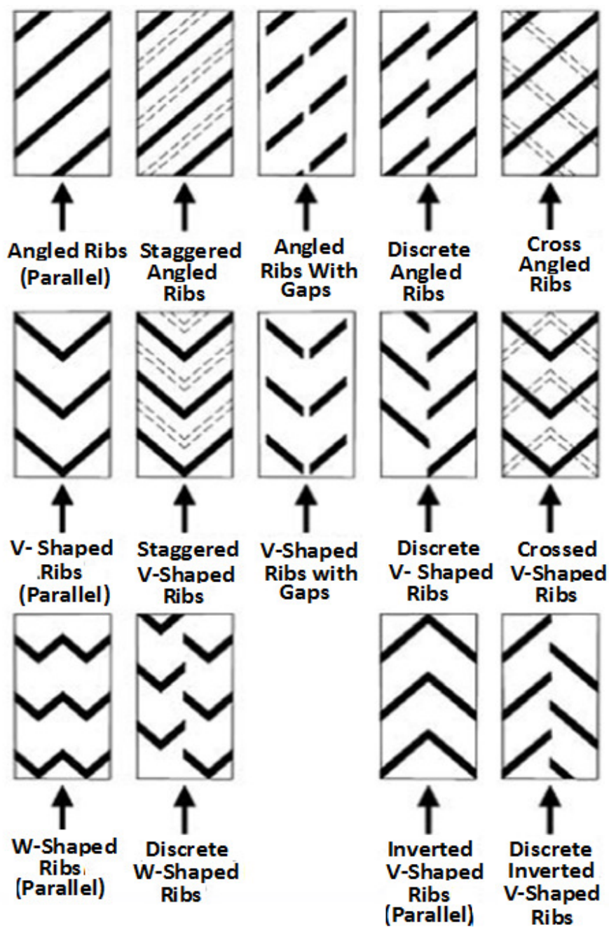
Figure 9.2: Advanced rib configuration in cooling channels
