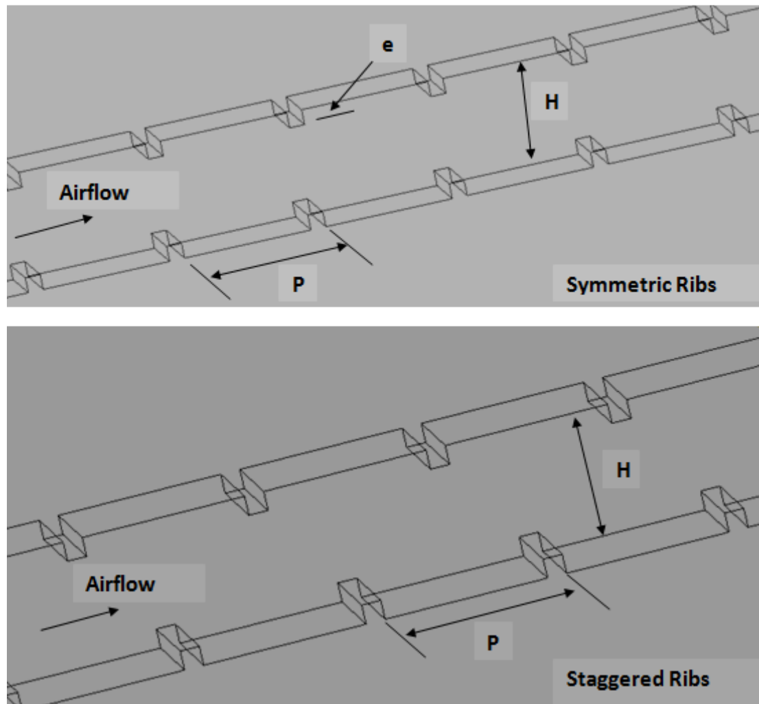
Figure 2.10: Symmetric and staggered ribs arranged on opposite wall of coolant passage.
