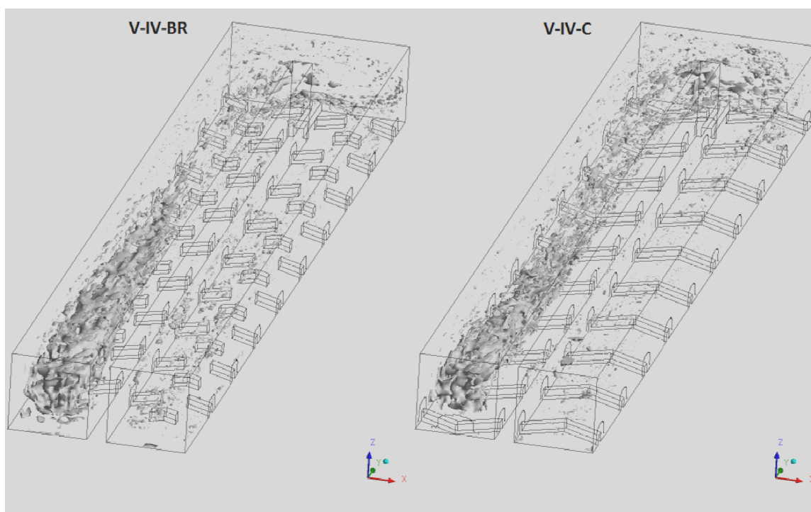
Figure 7.24: Isosurface for Vorticity: 379 s -1 (Re= 56000)
