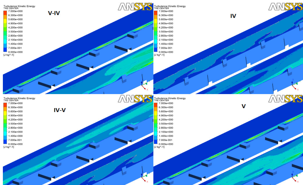
Figure 6.8: Broken Rib Turbulent Kinetic Energy @ x = 0.5D_h , @ x = 1.75D_h ( Re=21000 , k-\omega SST)
