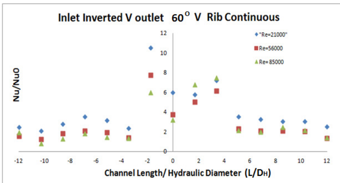
Figure 5.11 Comparison of 60° Inlet Inverted V and Outlet 60° V Rib continuous rib for different Reynolds Number
