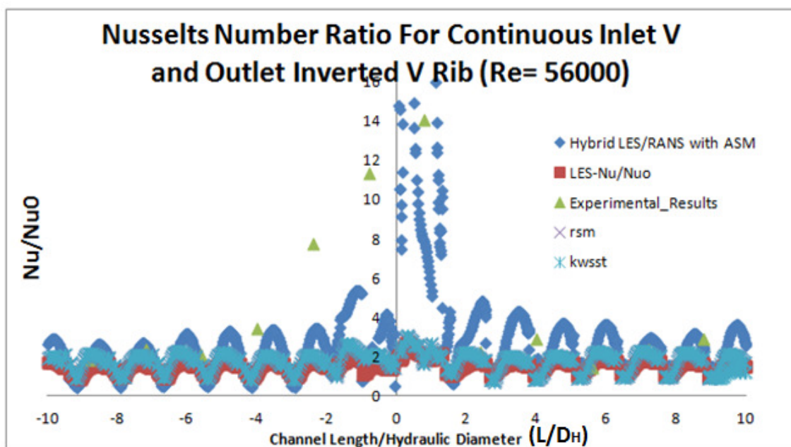
Figure 8.3 Inlet V and Outlet Inverted Continuous V Rib
