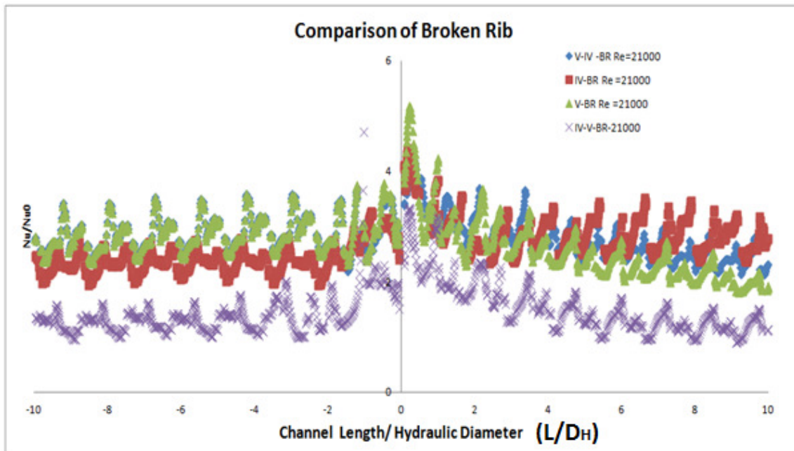
Figure B.23: Broken Rib k-\omega SST for all the rib arrangement
