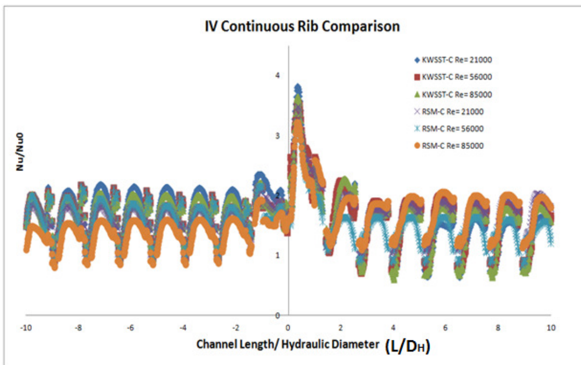
Figure B.20: Continuous Rib IV for k-\omega SST and RSM model
