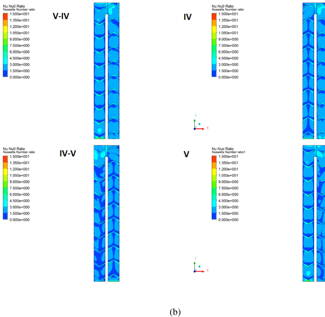
Figure B.7: Continuous Rib ( Re=21000 , RSM) (a) Surface Nusselt Number along wall
