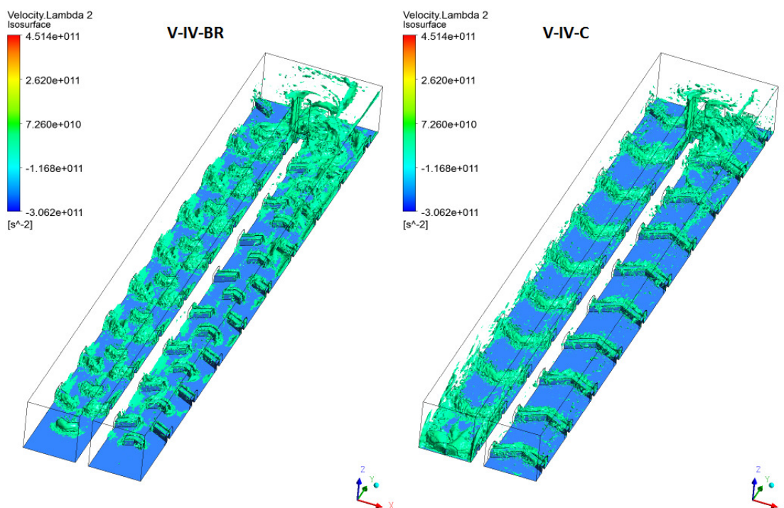
Figure 7.25: Isosurface for Velocity Lambda 2: 1.269\text{E}+06 \text{ s}^{-2} (Re= 56000)
