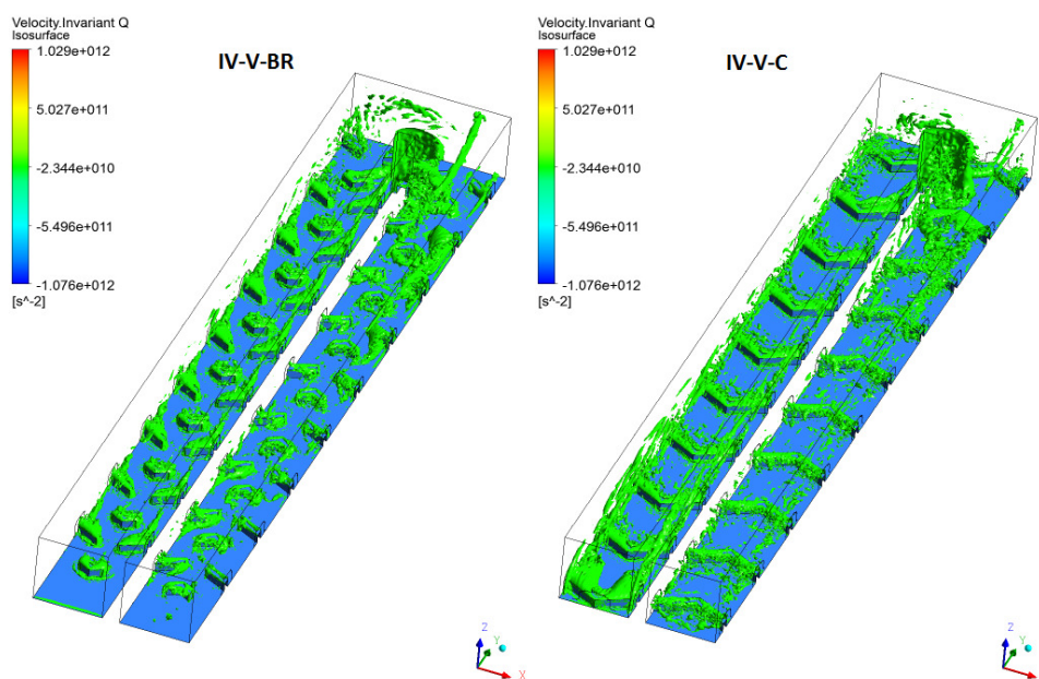
Figure 7.26: Isosurface for Velocity Invariant Q: 1.269\text{E}+06 \text{ s}^{-2} (Re= 56000)
