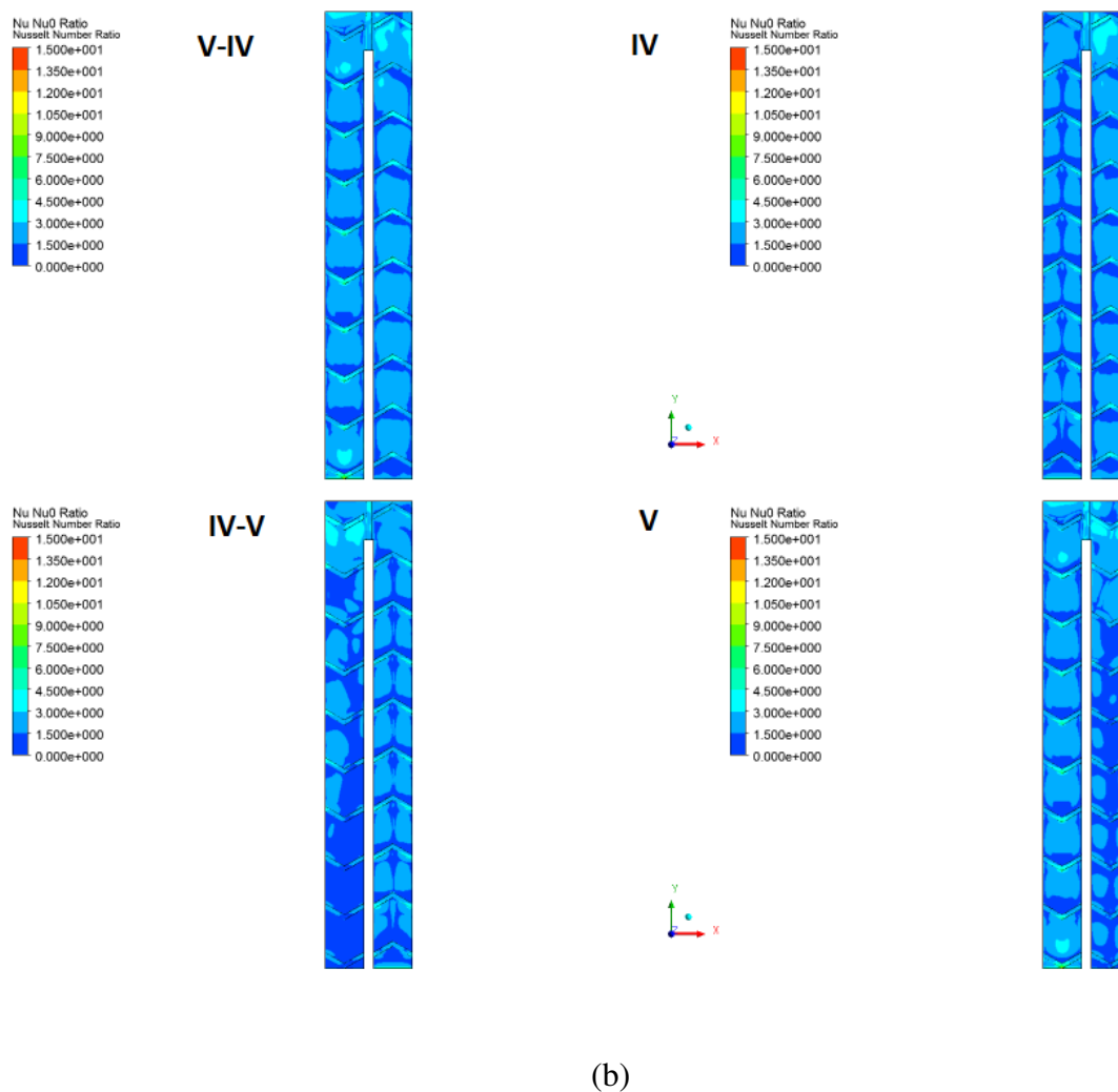
Figure B.5: Continuous Rib ( Re=56000 , k-\omega SST) (a) Surface Nusselt Number along wall (b) Surface Nusselt Number Ratio
