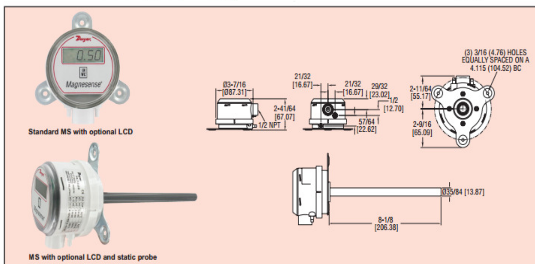
Figure A.10: Differential pressure transmitter to monitor pressure and velocity
