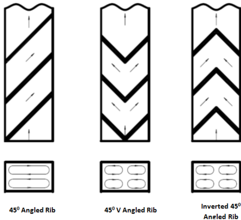
Figure 2.14: Secondary flow vortices induced by 45^\circ angled and 45^\circ V-Shaped ribs
