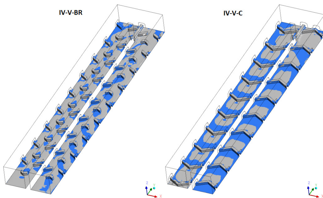
Figure 7.28: Isosurface for Vorticity: 3.516E+04 \text{ s}^{-1} (Re= 56000)
