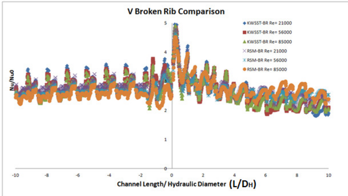
Figure B.17: Broken Rib V for k-\omega SST and RSM model
